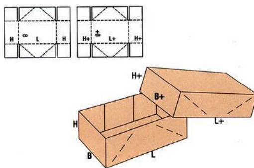
FEFCO 304
