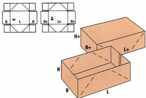
FEFCO 303
