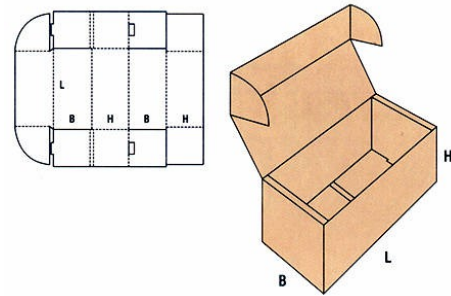
FEFCO 429
