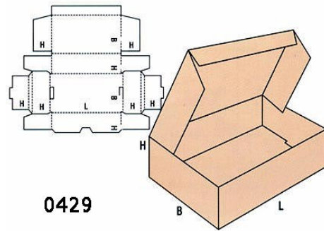
FEFCO 429
