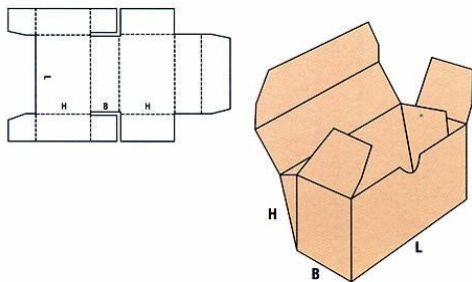
FEFCO 444
