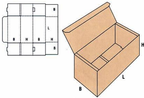
FEFCO 420
