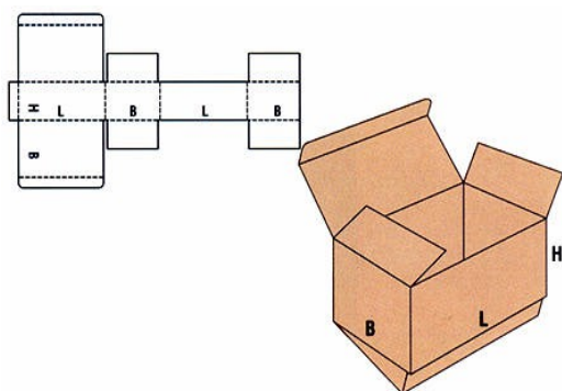
FEFCO 210
