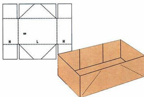
FEFCO 451
