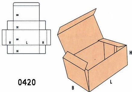
FEFCO 420
