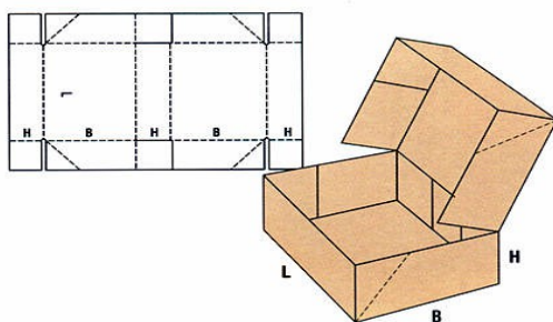
FEFCO 759
