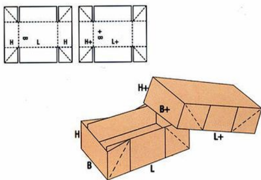
FEFCO 308
