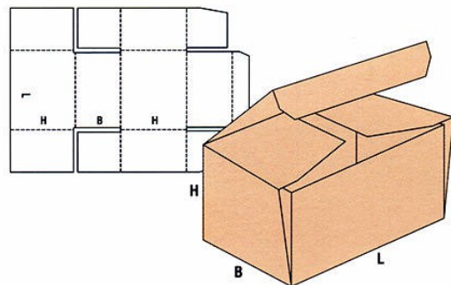
FEFCO 443
